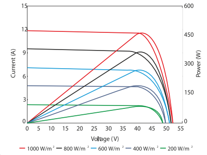
I-V Curves of PV Module (for Ref)
